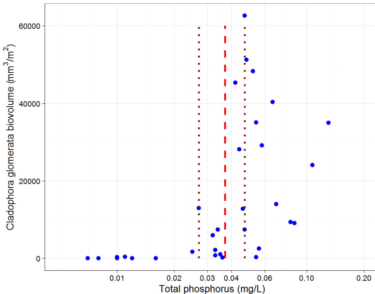
Figure ##. Two-year mean TP (April 2014-2016) vs. mean Cladophora glomerata biovolume from events 1, 3, 5, 6, 9, and 12. The dashed red line corresponds to 0.037 mg/L TP, whereas the dotted lines correspond to 0.027 and 0.047 mg/L TP, respectively.
