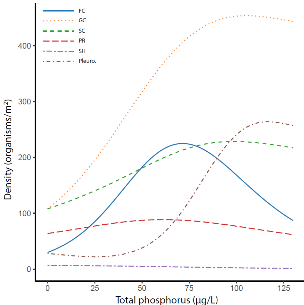
Figure ##. Mean responses of macroinvertebrate functional feeding groups to total phosphorus over the 2-year study period. FC=filtering collectors; GC=gathering collectors; SC=scrapers/grazers of algae, excluding pleurocerid snails; PR=predators; SH=shredders; Pleuro=pleurocerid snails.
