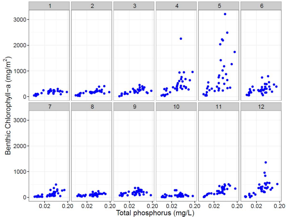
Figure ##. Relationship between benthic chlorophyll-a and 6-month mean TP across each event. Event 1 (June 2014) and 2 (August 2014) are based on 2 and 4 month mean TP values, respectively, because 6 month data was not available.
