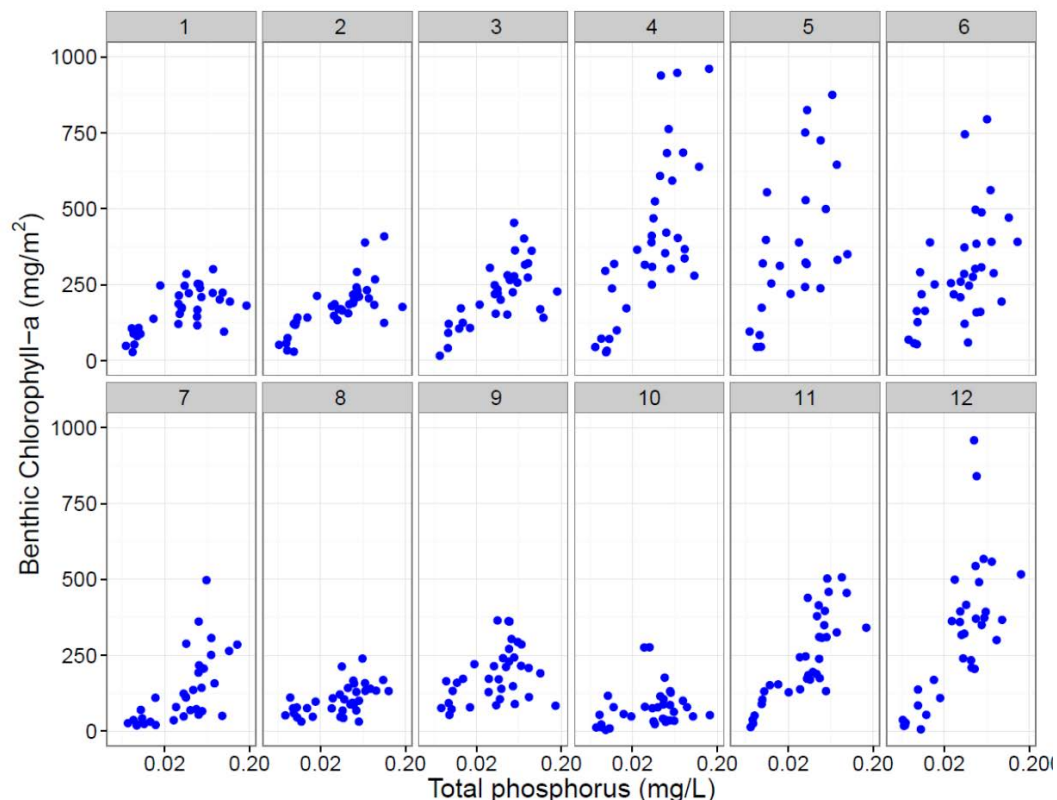
Figure ##. Relationship between benthic chlorophyll-a and 6-month mean TP across each event. This figure is identical to figure ## except that the y-axis was truncated at 1000 mg/m 2 so that the relationship between TP and benthic chlorophyll-a during periods outside the massive Cladophora blooms could be better visualized.
