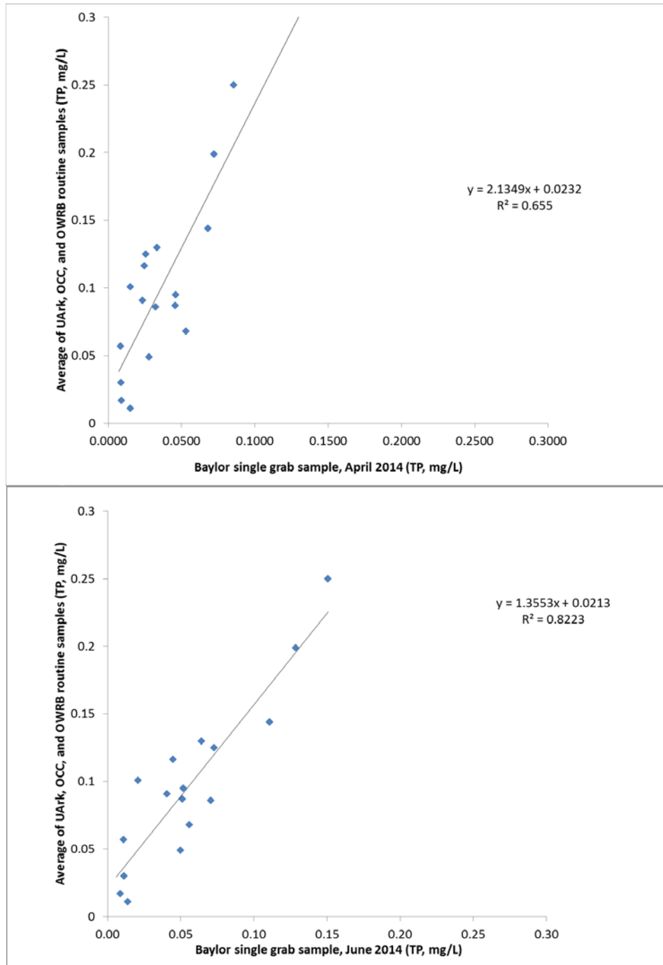
Figure ##. Relationship between single grab samples collected by Baylor in April (upper panel) and June (lower panel) 2014 to mean TP over 1-2 years prior to the Baylor samples from intensive sites monitored by the Oklahoma Conservation Commission (OCC), Oklahoma Water Resources Board (OWRB), and the University of Arkansas (UA).
