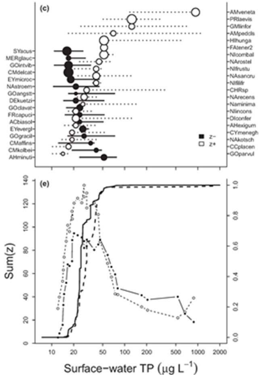
Figure 5. Example of output from Threshold Indicator Taxa Analysis (TITAN). In this example from a study conducted in wadeable streams in central Texas (Taylor et al. 2014), species with negative responses to total phosphorus are shown as filled symbols, whereas species that increased in response to TP are shown as open circles (upper panel). The location of the symbols corresponds to the level of TP resulting the greatest change in the frequency and abundance of each taxon (the change point) and the horizontal lines span the lower to upper quantile intervals (uncertainty). The lower panel illustrates the sum of the responses of the pure and reliable threshold indicator taxa. Sumz- (negative responding taxa) sharply peaks at 0.021 mg/L TP with lower and upper quantile limits of 0.016-0.052 mg/L. Sumz+ (positive responding taxa) sharply peaked at 0.028 (0.018-0.048) mg/L TP. Both results are indicative of a significant shift in species composition between ~0.02-0.05 mg/L TP.
