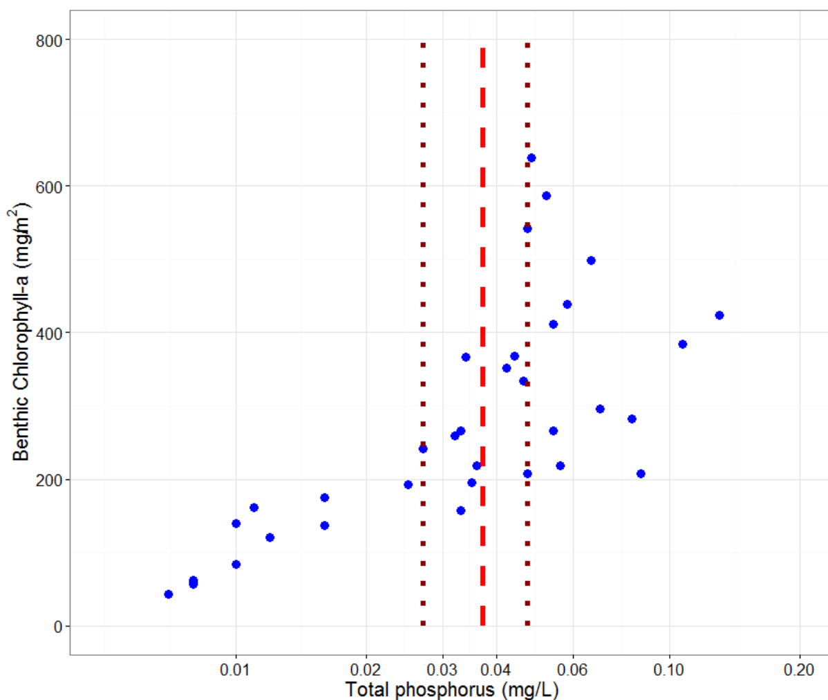
Figure ##. Two-year mean TP (April 2014-2016) vs. 2 year mean benthic chlorophyll-a. The dashed red line corresponds to 0.037 mg/L TP, whereas the dotted lines correspond to 0.027 and 0.047 mg/L TP, respectively.
