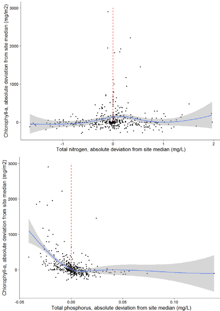
Figure ##. Plots of benthic chlorophyll-a in response to TN (upper) and TP (lower) deviations from site medians. The upper panel shows that the largest chlorophyll-a values were associated with mostly normal TN concentrations, with no relationship to benthic chlorophyll-a. The lower panel shows that almost all of the high chlorophyll-a levels corresponded to sharp reductions in TP. The fitted relationship shows that as TP levels were increasingly reduced, chlorophyll was at its highest. TP levels that are far above the median appear to be related to below normal levels of benthic chlorophyll-a.
