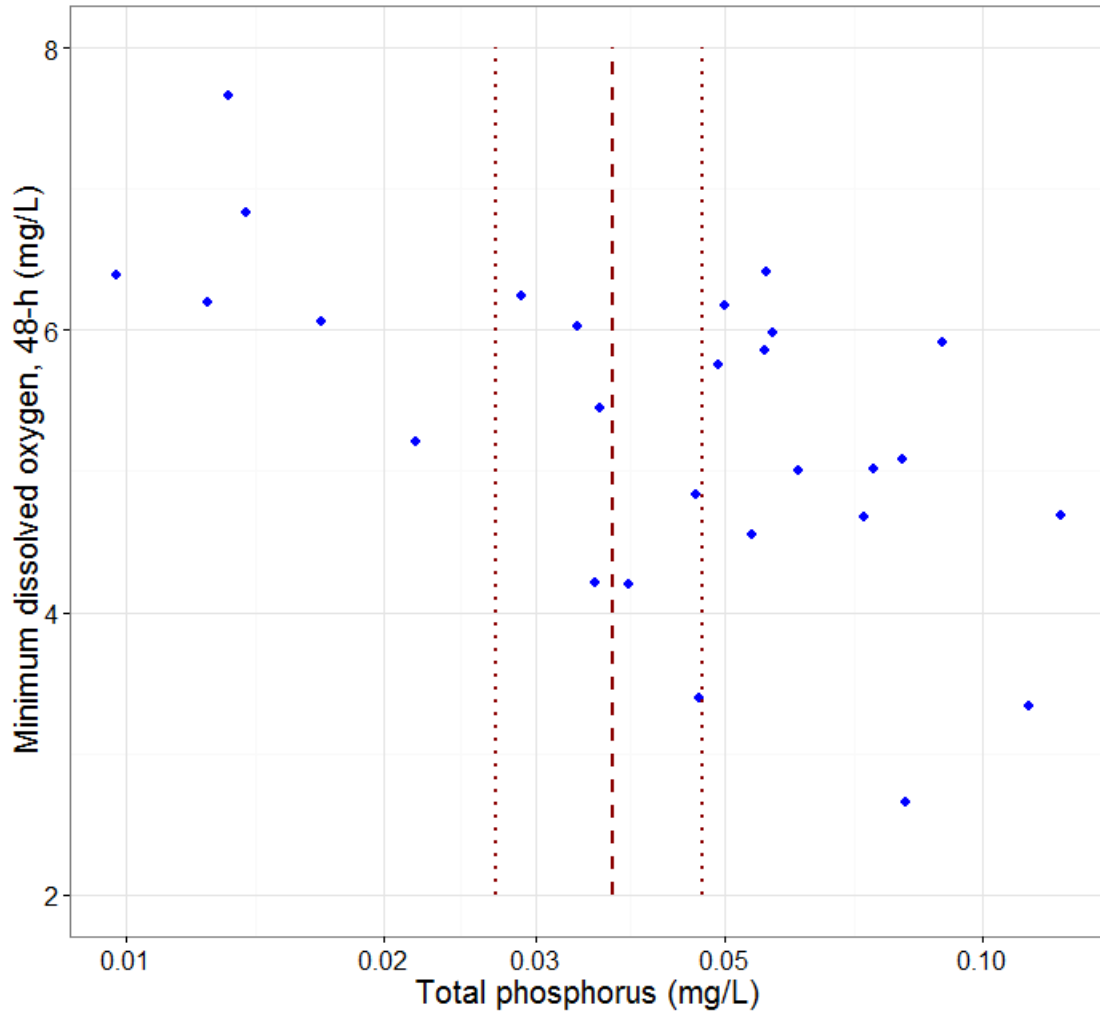
Figure ##. Minimum 48-h dissolved oxygen in August 2014 in response to mean 6-month total phosphorus. The red vertical dashed line corresponds to 0.037, whereas the dotted red vertical lines correspond to 0.027 and 0.047 mg/L, respectively.
