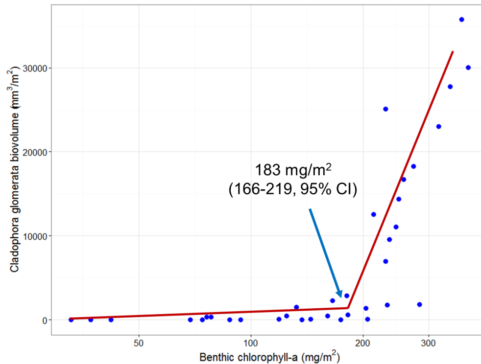
Figure ##. Results of segmented regression relating mean Cladophora glomerata biovolume to mean benthic chlorophyll-a during year 1 (upper panel) and year 2 (lower panel). Year 1 data represents a year with very stable flows overall, whereas year 2 represents a wet year with many scouring flows, including an historic flood.
