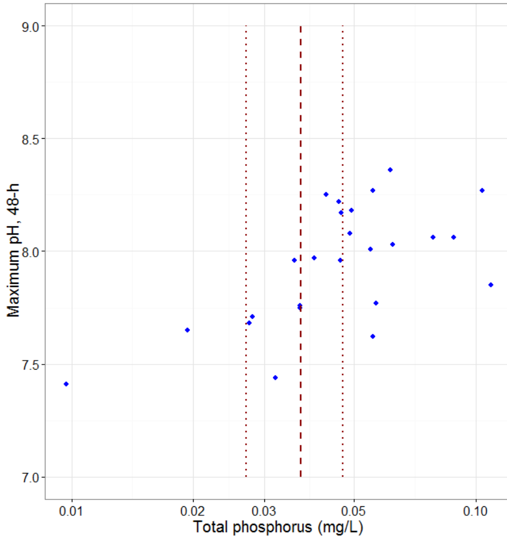
Figure ##. Maximum 48-h pH in September 2015 in response to mean 6-month total phosphorus. The red vertical dashed line corresponds to 0.037, whereas the dotted red vertical lines correspond to 0.027 and 0.047 mg/L, respectively.
