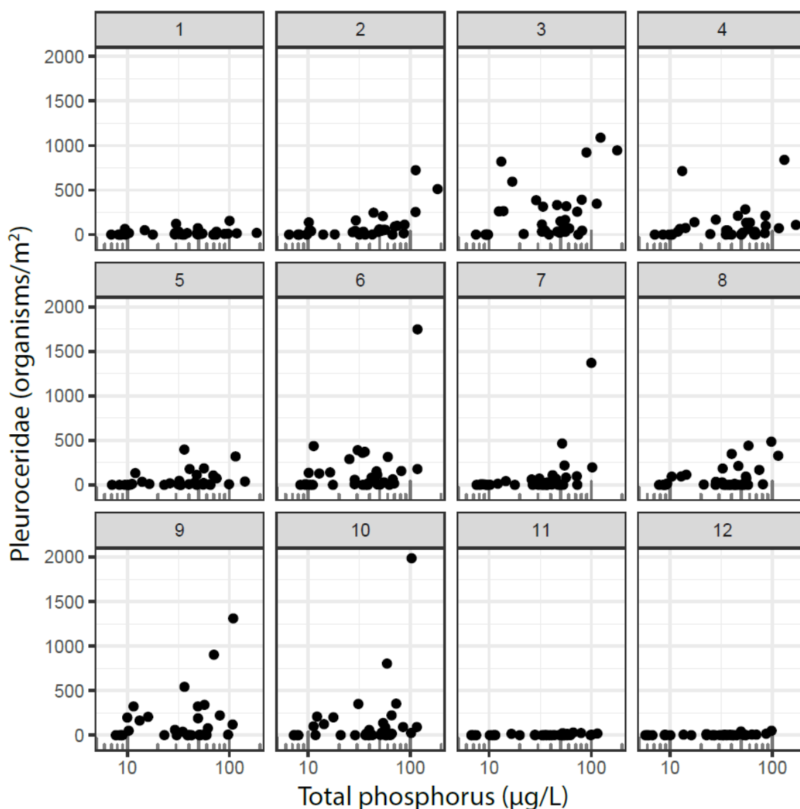
Figure #. Densities of pleurocerid snails versus 6 month mean TP across the 2-year study period. Numbers in the upper panels are event numbers (1-12).
