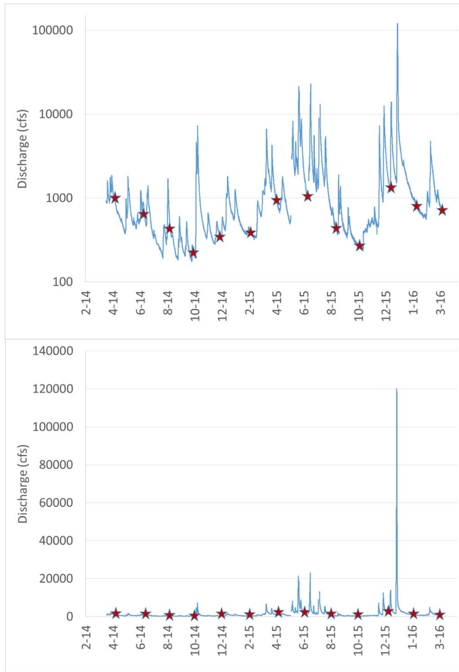
Figure ##. Daily mean discharge at USGS gage 07196500, Illinois River at Tahlequah, from April 2014-2016. Location of the stars indicates the approximate timing of sampling. Discharge is log-scaled in the upper panel, whereas an untransformed scale is used in the lower panel. The huge peak in the lower panel corresponds to the historic flood event in late December 2015.
