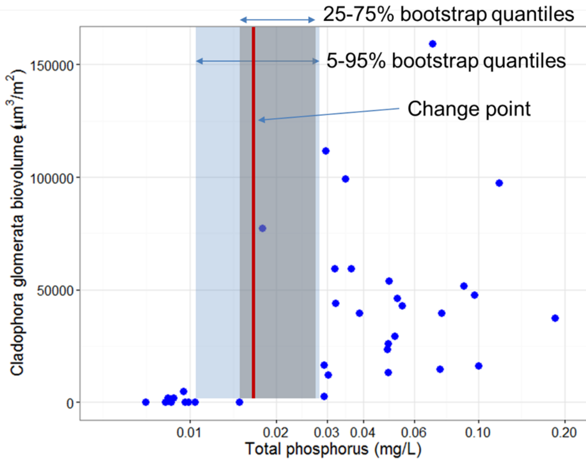
Figure ##. Change point threshold approach based on splitting the data at a TP value that corresponds to the largest change in the response (in this case, biovolume of Cladophora , the primary nuisance species in the Designated Scenic Rivers). Here, the data are 2 month TP versus instantaneous Cladophora biovolume from June 2014.
