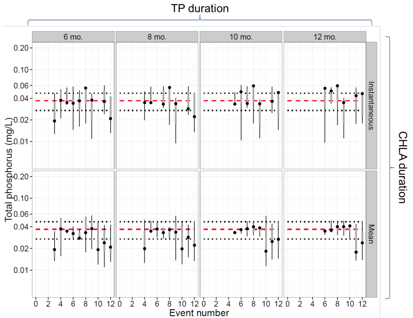
Figure ##. Total phosphorus change points in relation to benthic chlorophyll a. The columns represent 6, 8, 10, and 12 month TP durations, whereas the rows separate instantaneous and mean chlorophyll-a. Points correspond to the observed change point, gray bars span the 25-75% bootstrap quantiles, and black bars span the 5-95% bootstrap quantiles. The dashed red line is 0.037 mg/L TP, whereas the upper and lower dotted lines correspond to 0.027 and 0.047 mg/L. Results for 2 and 4 month TP are not shown, but are included in tables ## and ##.
