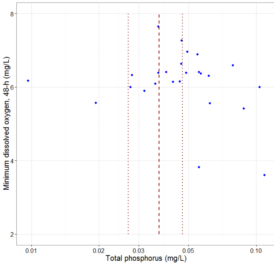
Figure ##. Minimum 48-h dissolved oxygen in September 2015 in response to mean 6-month total phosphorus. The red vertical dashed line corresponds to 0.037, whereas the dotted red vertical lines correspond to 0.027 and 0.047 mg/L, respectively.
