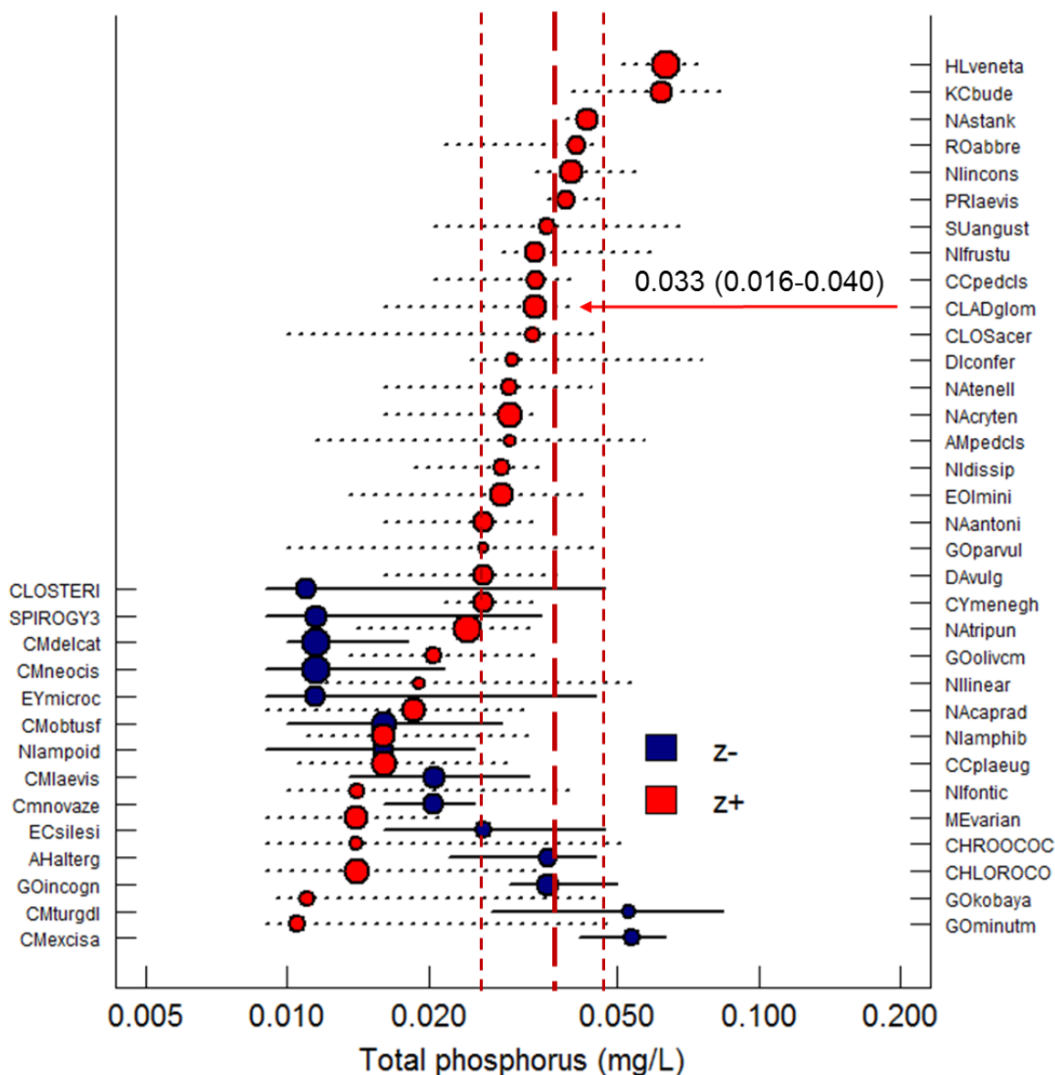
Figure ##. Results of TITAN using two-year mean TP (April 2014-2016) as the predictor vs. mean biovolume of all taxa that occurred at least 3 times from events 1, 3, 5, 6, 9, and 12. Shown are pure and reliable threshold indicator taxa. Negative responding taxa are listed on the left y-axis and marked by dark blue points, whereas positive responding taxa are on the right y-axis and marked by red points. Points are located at change point. Error bars represent the 5-95% bootstrap quantile intervals. The community-level threshold for negative-responding taxa (sumz-) was 0.021 (0.010-0.025) mg/L, whereas the positive-responding community threshold was also 0.021 mg/L, but had higher bootstrap quantile intervals (0.016-0.033). The vertical, red dashed line corresponds to 0.037 mg/L TP, whereas the vertical dotted lines correspond to 0.027 and 0.047 mg/L TP, respectively.
