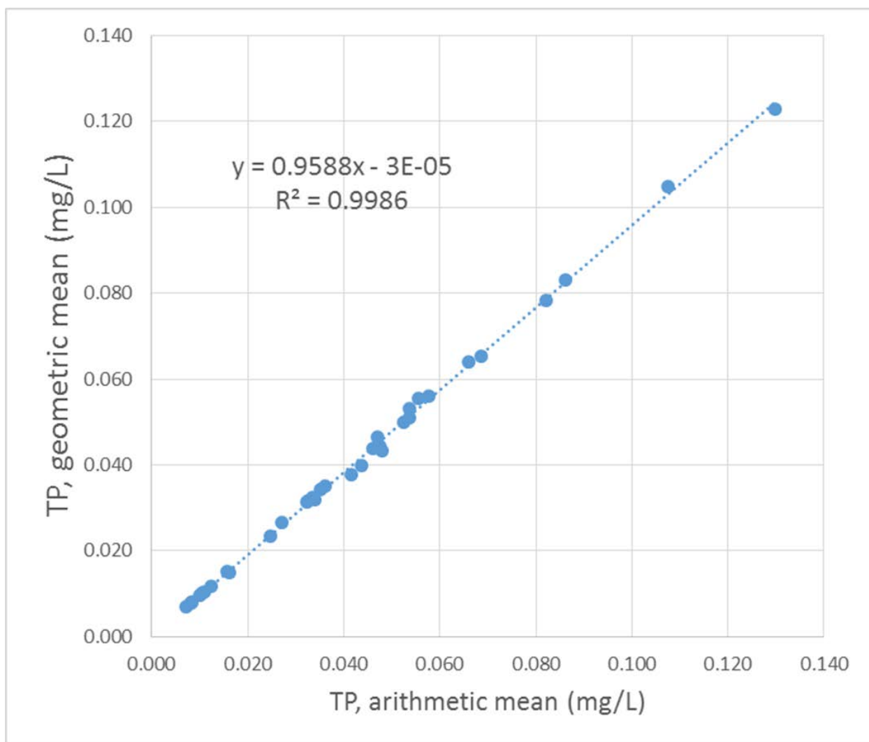
Figure ##. The relationship between geometric and arithmetic mean total phosphorus concentrations from the 35 study sites from April 2014 through April 2016 (n=13).
