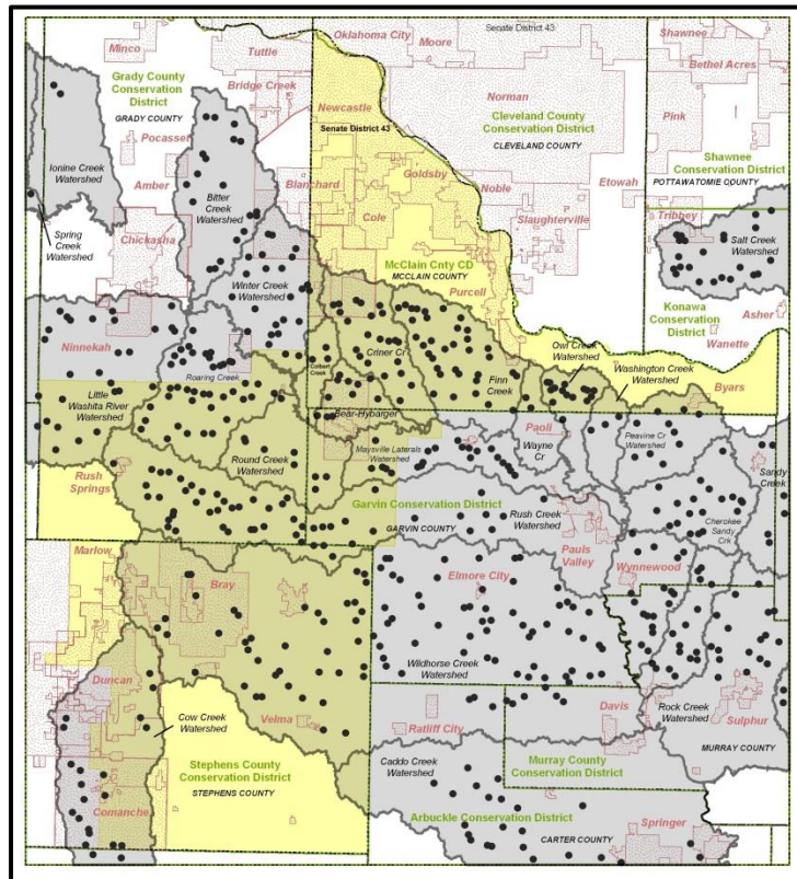
There are 237 flood control dams in 15 watershed projects in Senate District 43.
